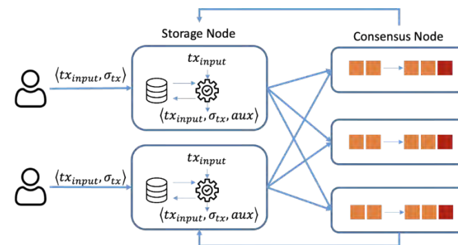
Stateless Blockchain
