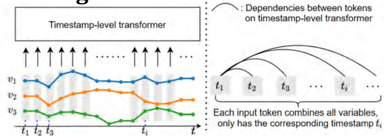
(a) LHS: the timestamp-level transformer; RHS: the dependencies (lines) of all tokens (timestamps) to first token learned by the transformer. The input token of timestamp-level transformer combines all variables at one timestamp, the transformer only captures the temporal dependencies.
