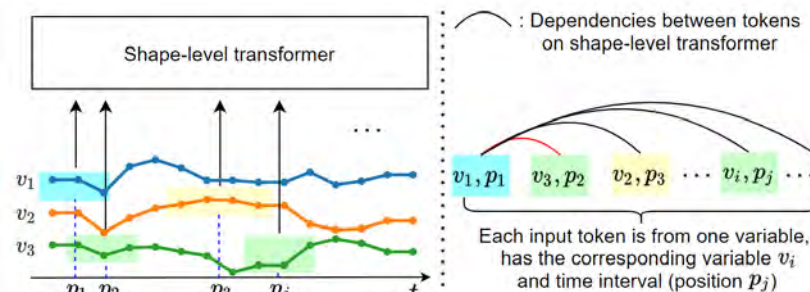
(b) LHS: the shape-level transformer; RHS: the dependencies (lines) of all tokens (shapes) to first token learned by the transformer. The input token of shape-level transformer is from one variable v_i with the corresponding time interval (position p_j ). By capturing the dependencies between shapes, the dependencies of variables and positions are learned. The red line denotes the dependencies between v_1 and v_3 .
